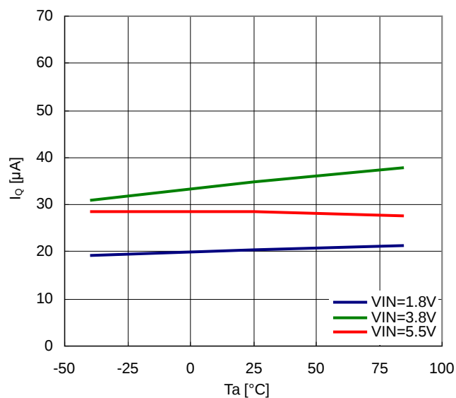
10) Quiescent Current vs. Temperature
