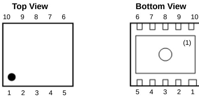
RP517K [DFN(PL)2527-10] Pin Configuration
