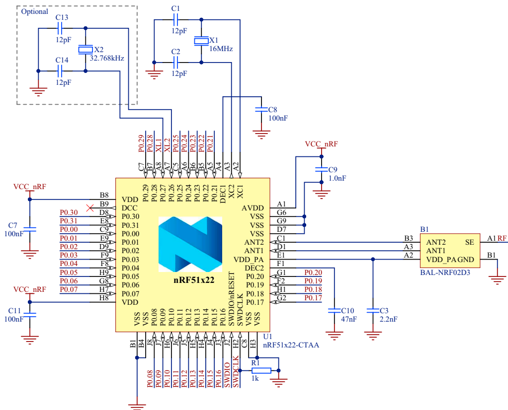
Figure 42 CTAA WLCSP with internal LDO setup
