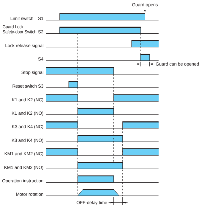
Timing Chart
