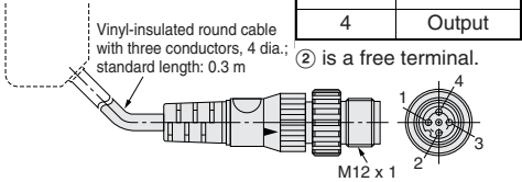
Connector relay models (E3Z-□□-M1J)
