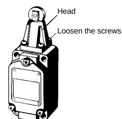
Example of roller plunger switches
