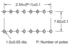
PCB Dimensions (Reference) (Top View)
