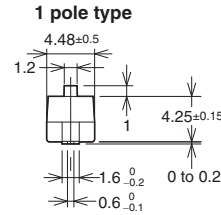
Flat actuator Standard
