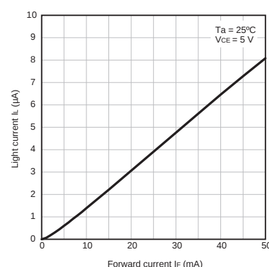
Fig 3. Light Current vs. Forward Current Characteristics (Typical)
