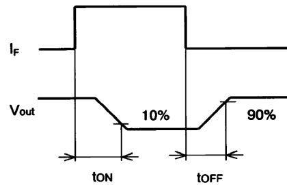
Timing Chart
