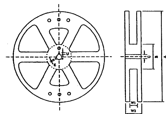
Reel Figuration
