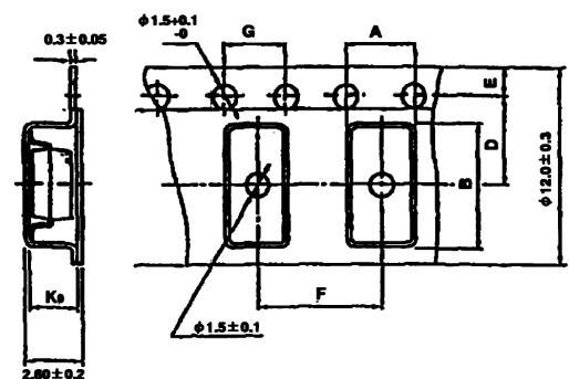
Type Figuration
