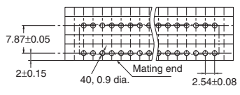
Mounting holes (bottom view)
