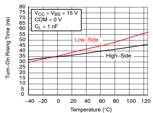
Figure 9. Turn-On Rising Time vs. Temperature
