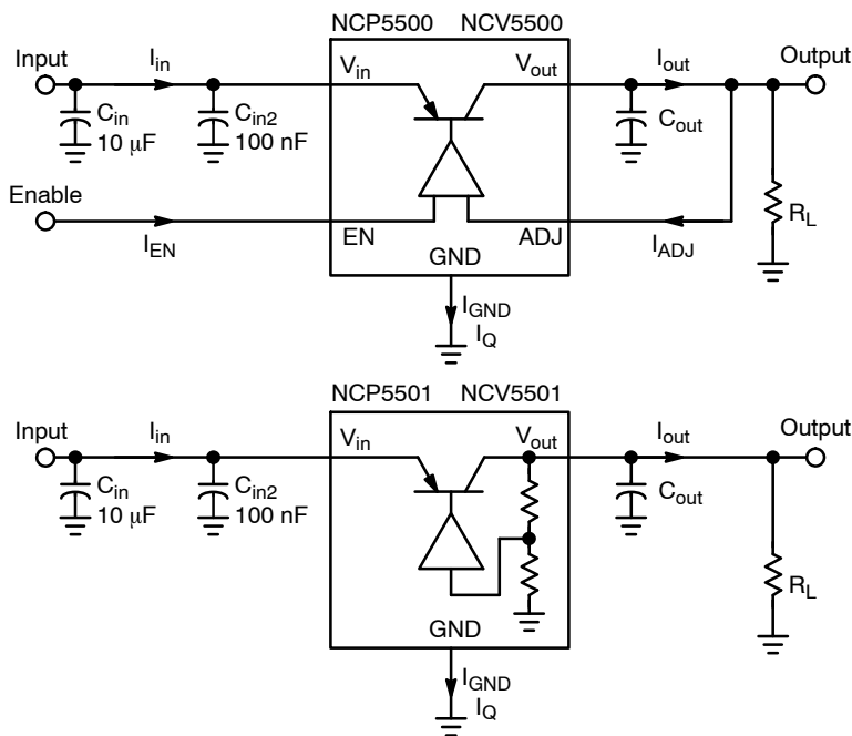
Figure 21. Measuring Circuits
