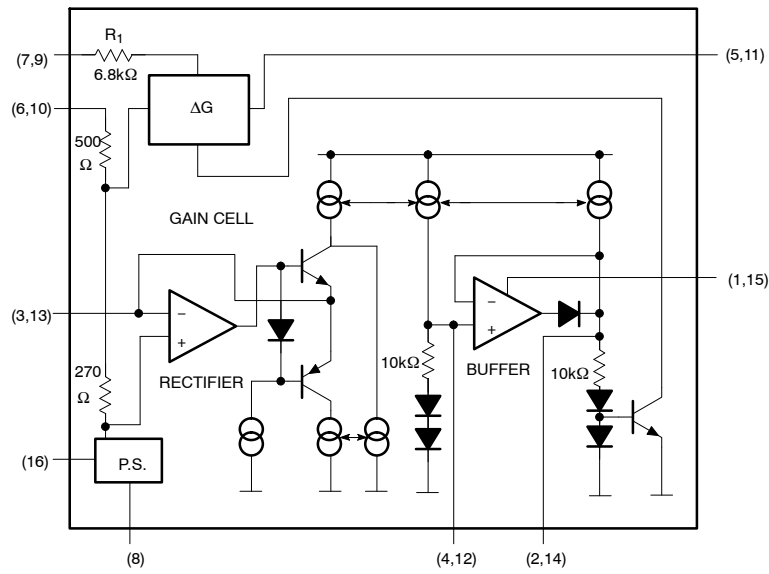
Figure 1. Block Diagram
