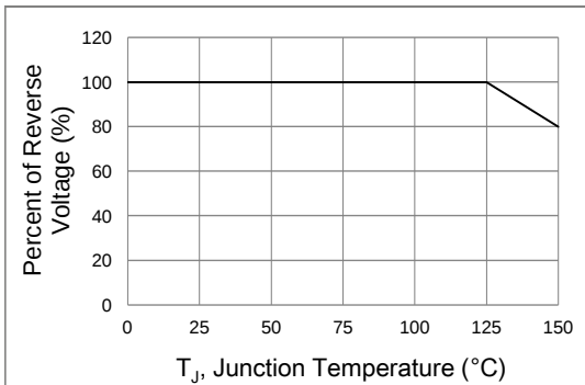
Fig.11 Operating Temperature Derating Curve
