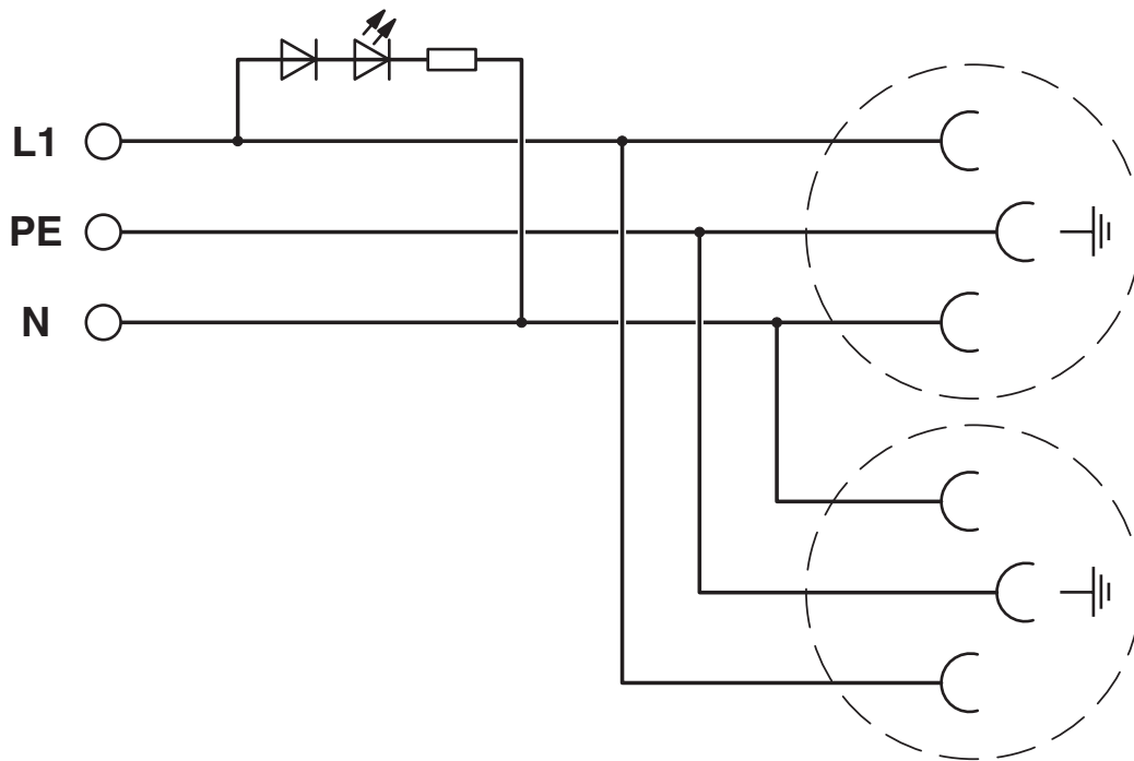
Circuit diagram
