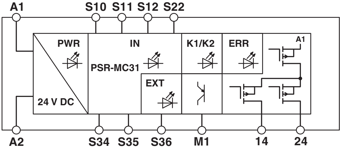
Block diagram
