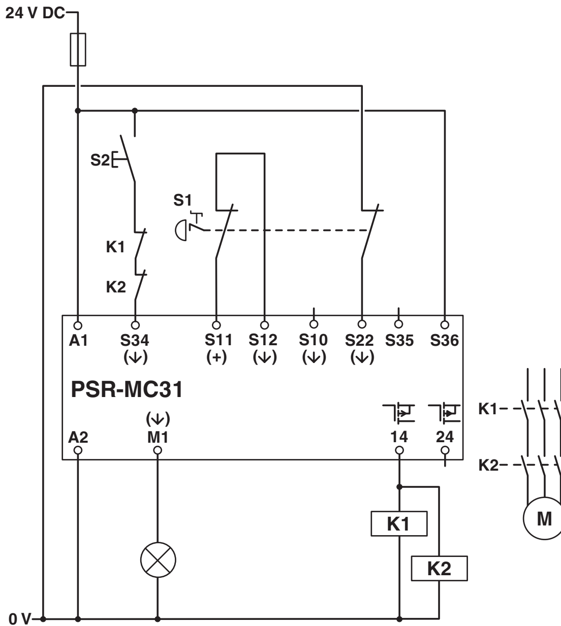
Circuit diagram
