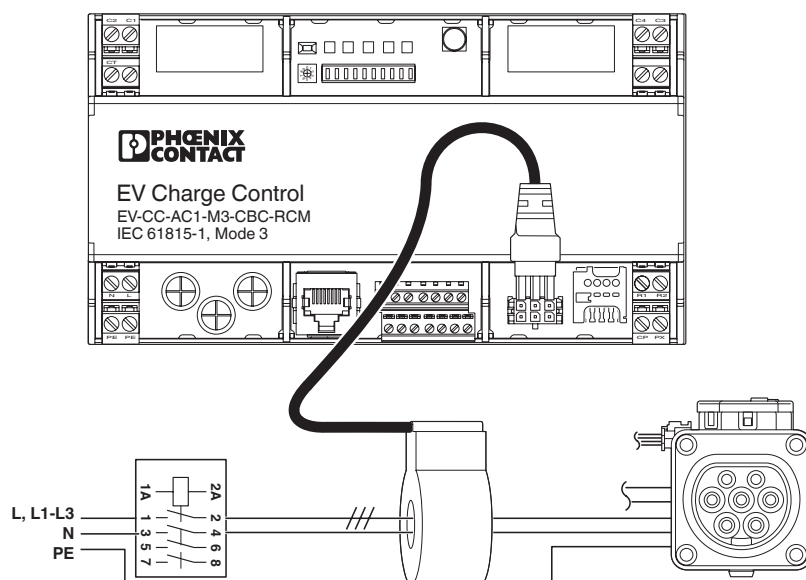
Connection diagram
