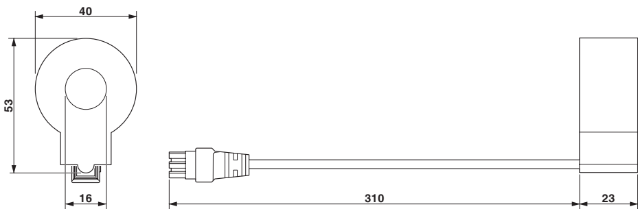
Dimensional drawing
