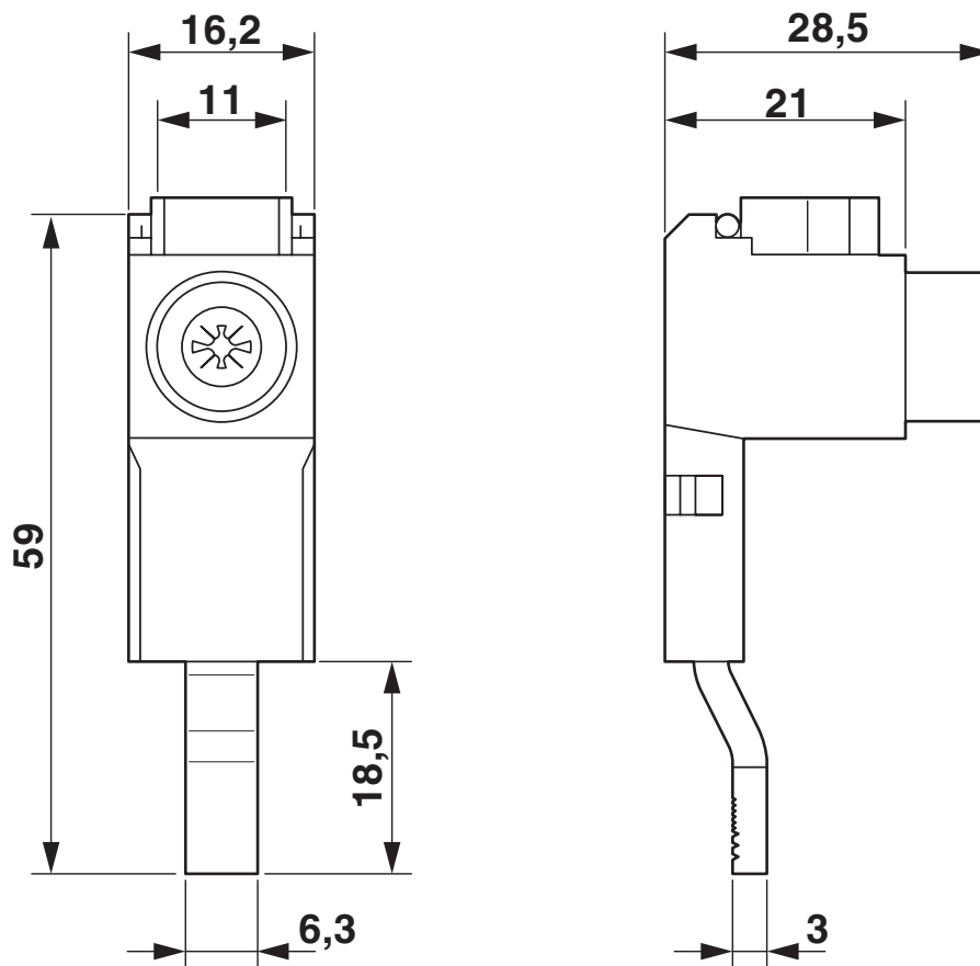
Dimensional drawing
