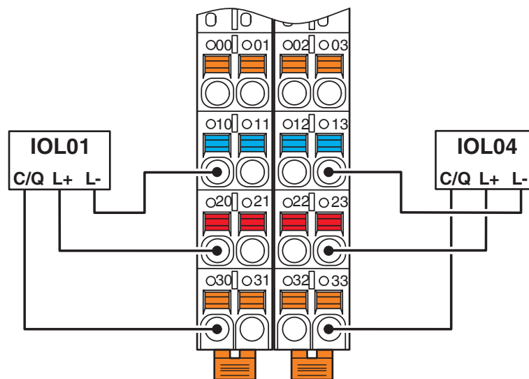
Connection diagram
