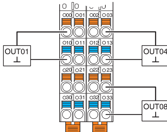
Connection diagram
