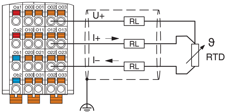
Connection diagram
