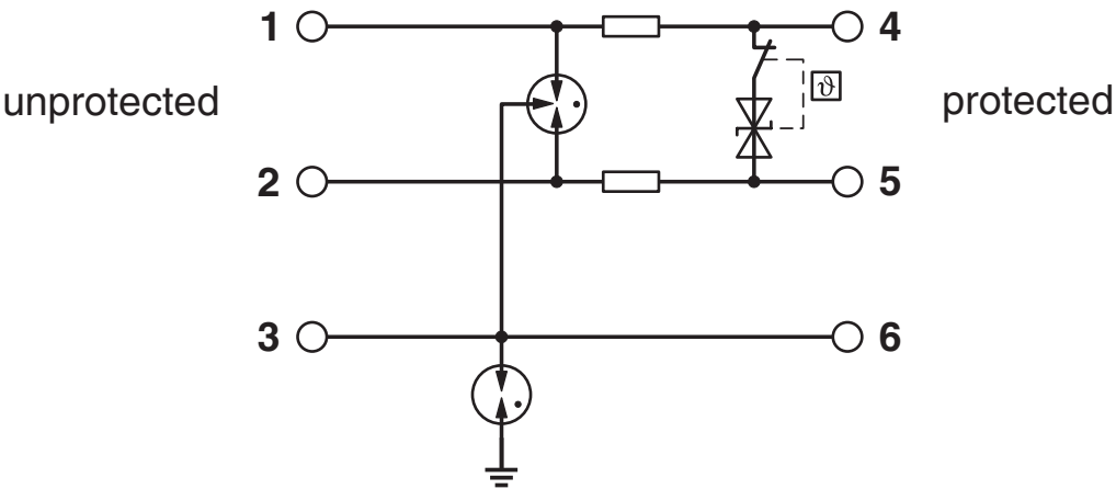
Circuit diagram
