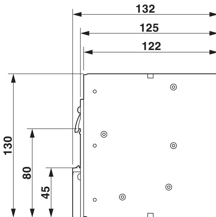
Dimensional drawing
