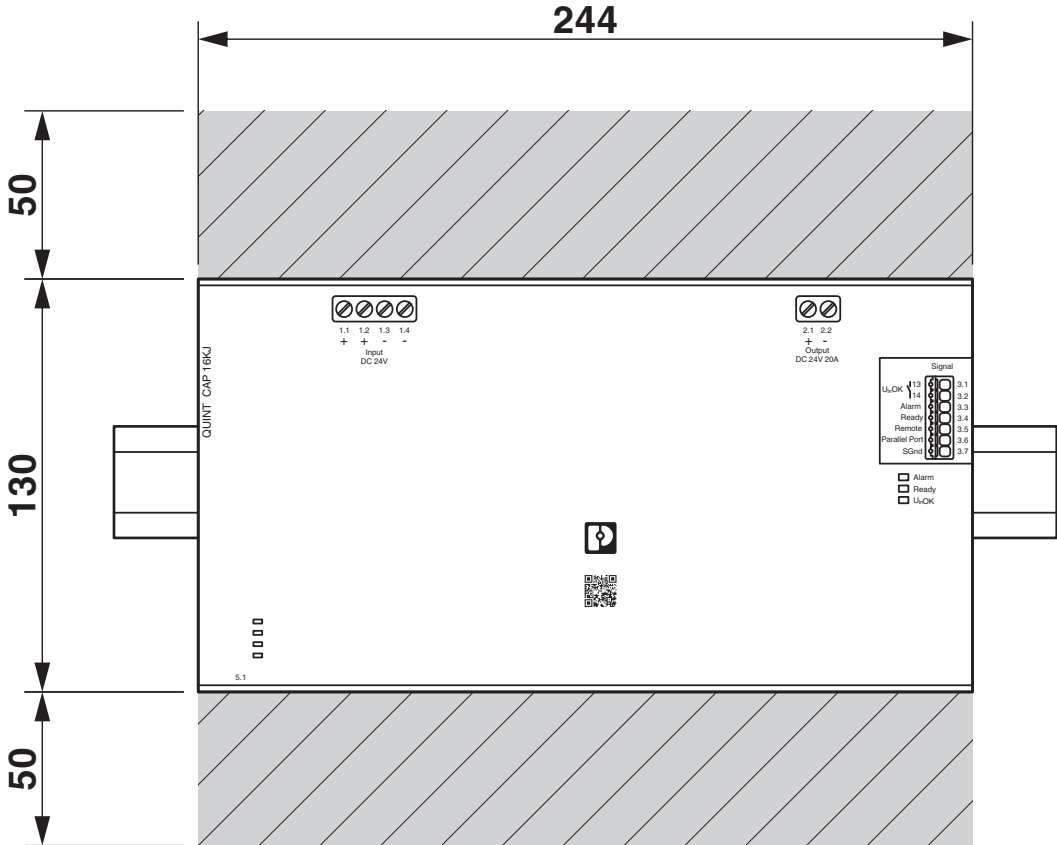
Device dimensions (dimensions in mm)
