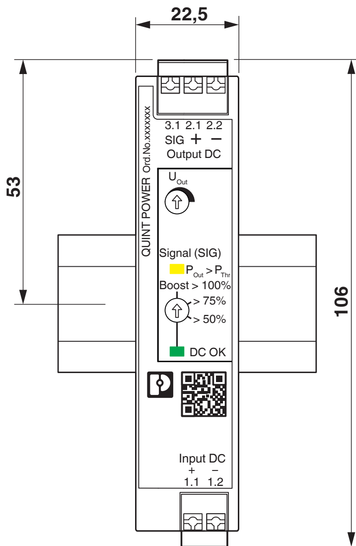
Dimensional drawing
