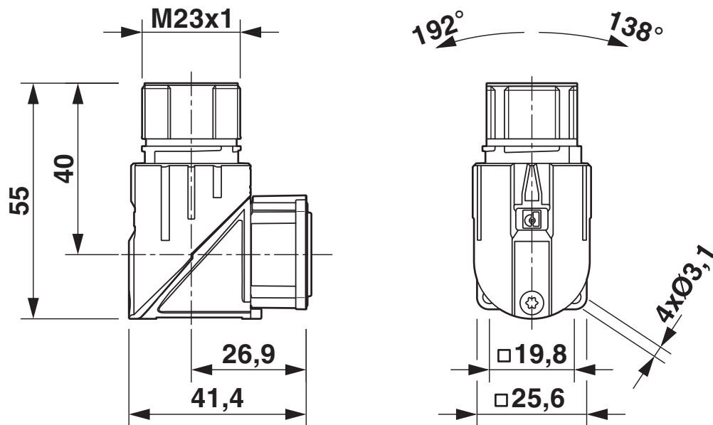
Dimensional drawing
