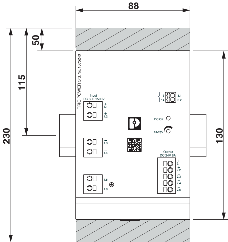
Dimensional drawing
