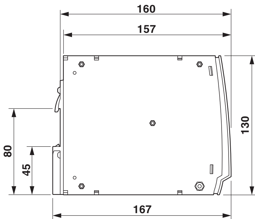
Dimensional drawing
