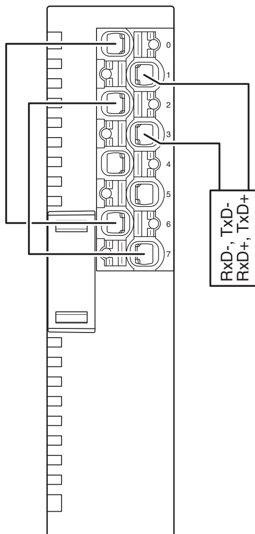
Connection diagram
