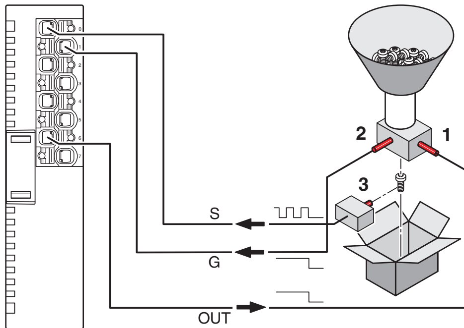
Connection diagram
