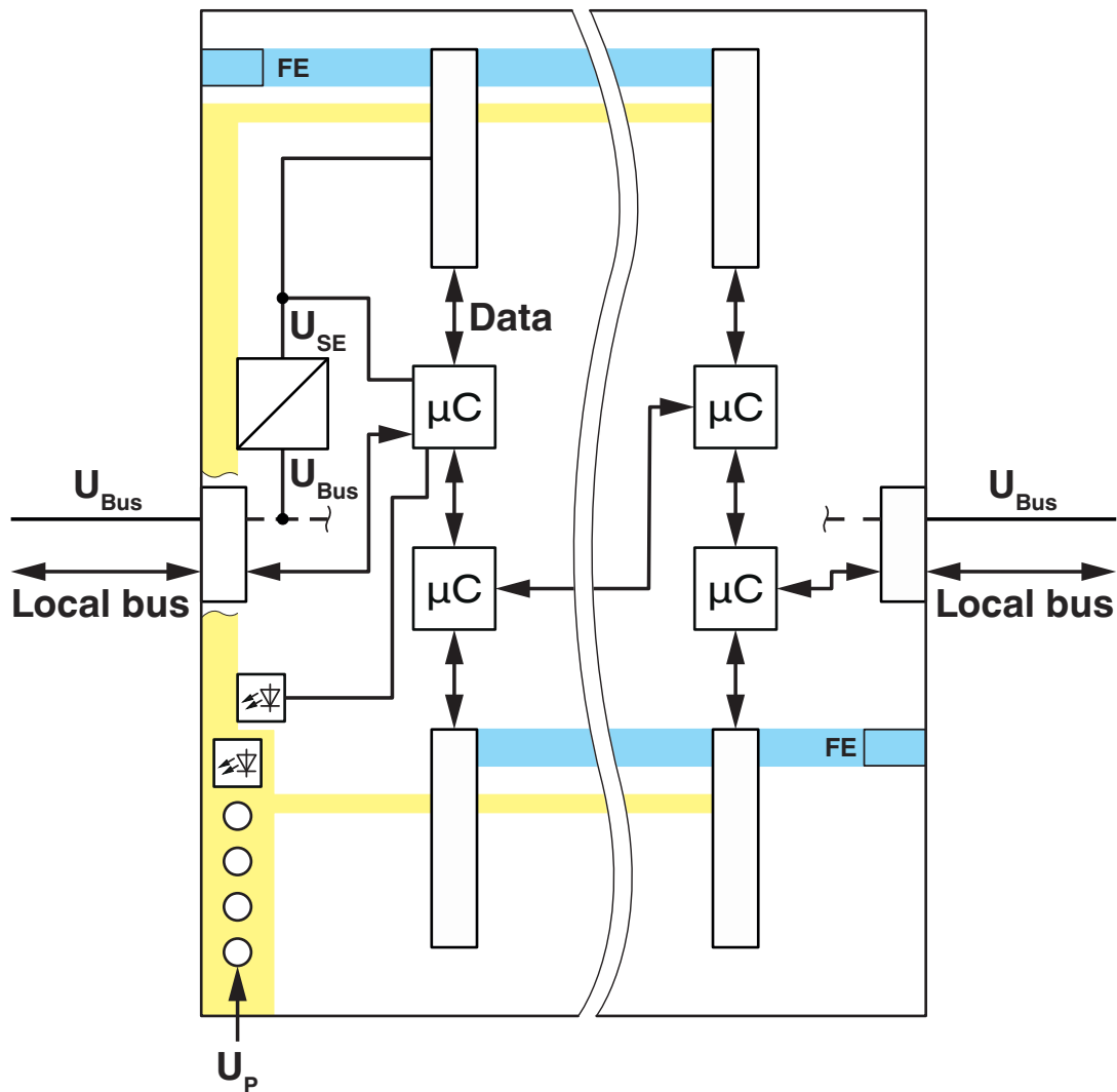
Block diagram
