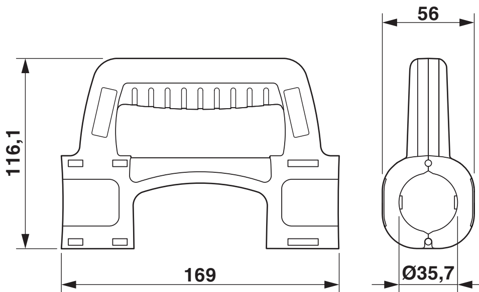
Dimensional drawing
