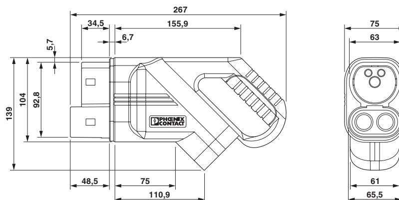
Dimensional drawing
