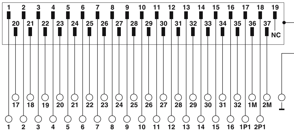
Circuit diagram
