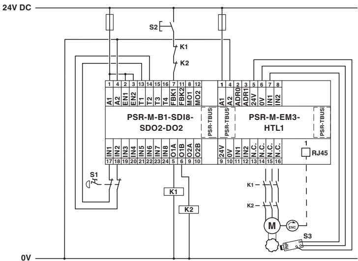
Application drawing
