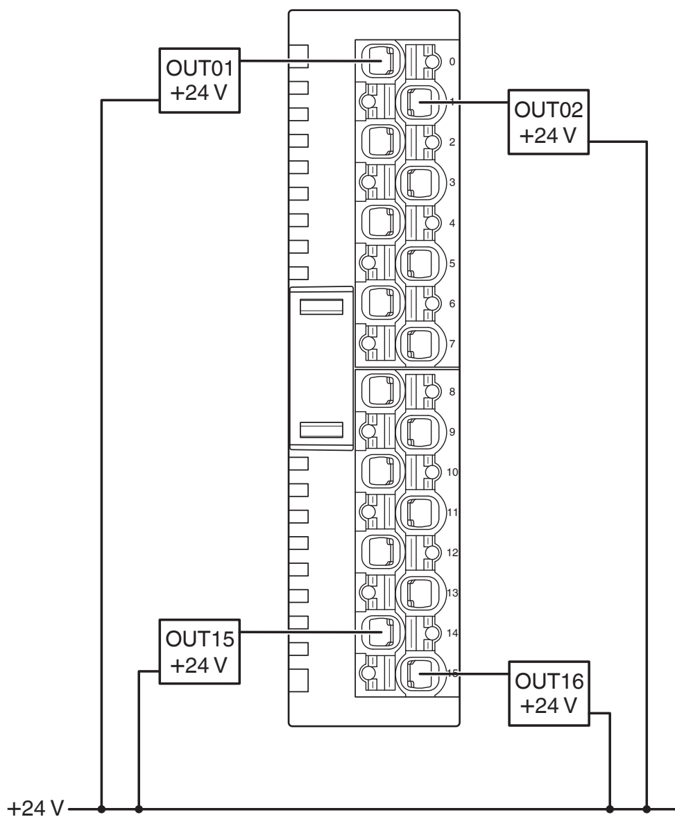
Connection diagram
