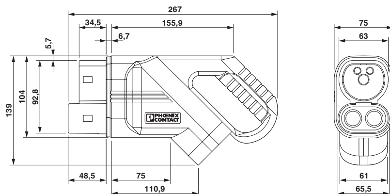
Dimensional drawing
