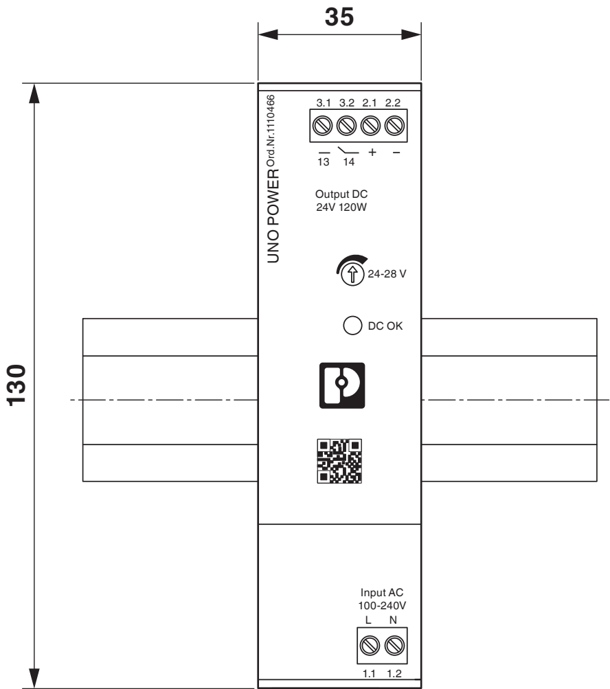
Dimensional drawing
