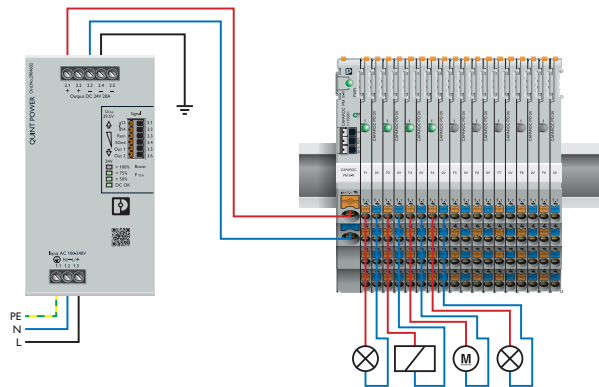
Application drawing
