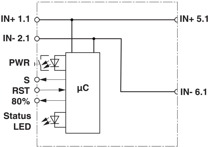
Block diagram
