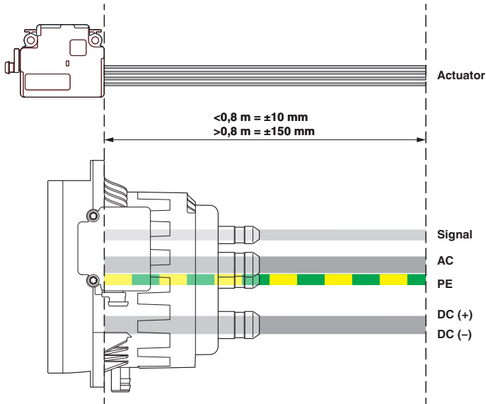
Dimensional drawing
