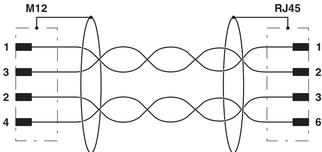
Circuit diagram
