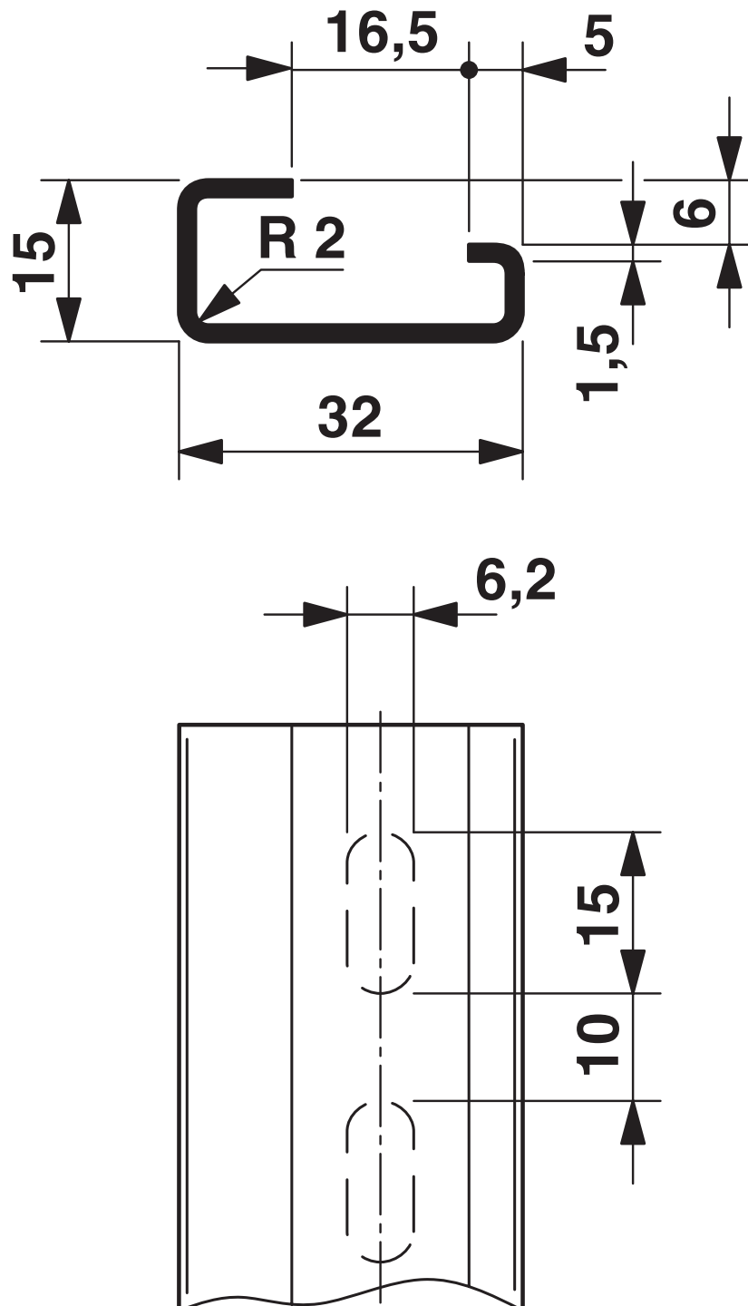
Dimensional drawing
