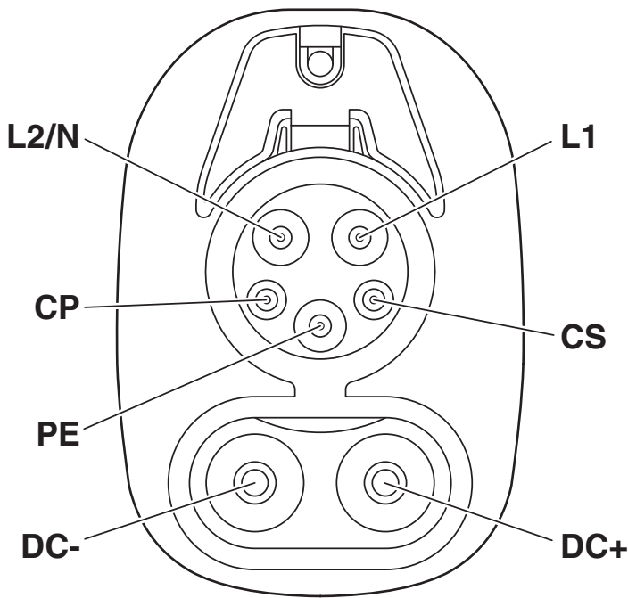
Connection diagram
