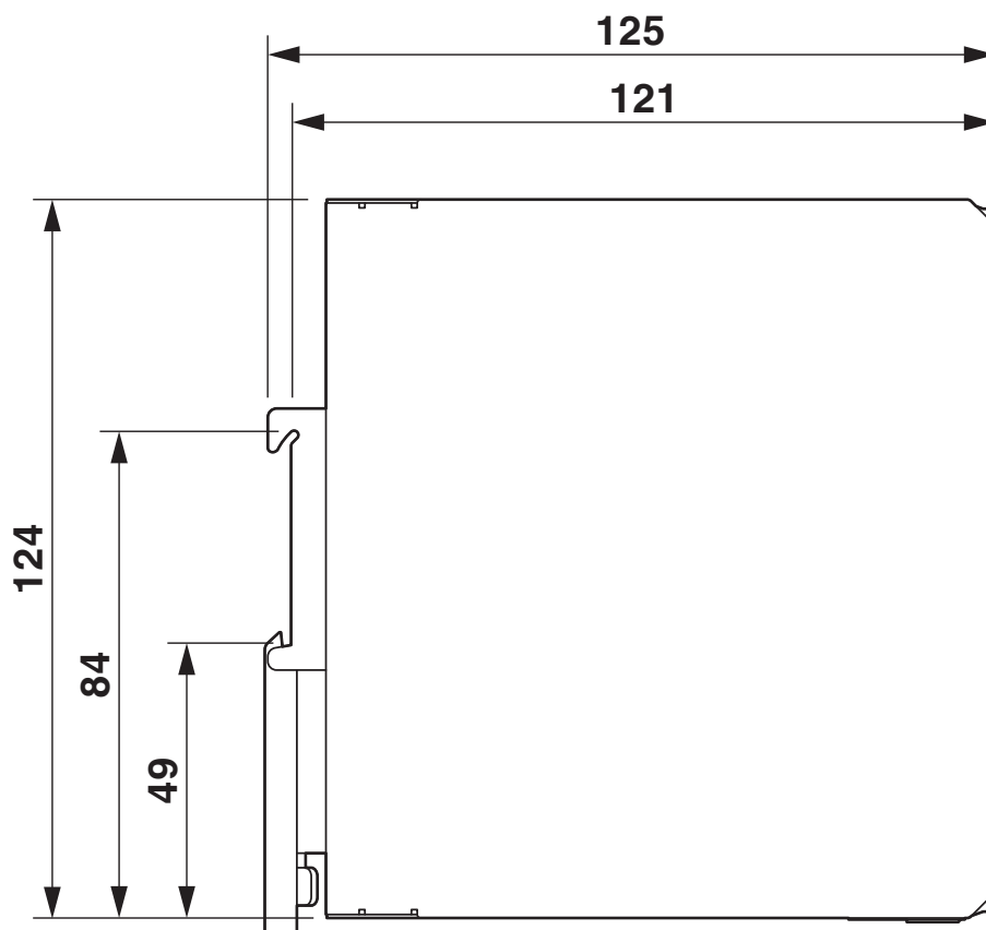
Dimensional drawing
