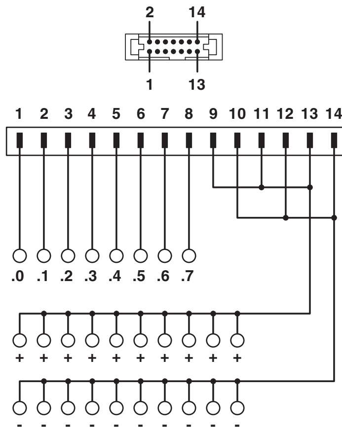
Circuit diagram
