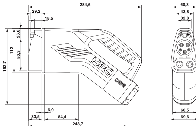
Dimensional drawing
