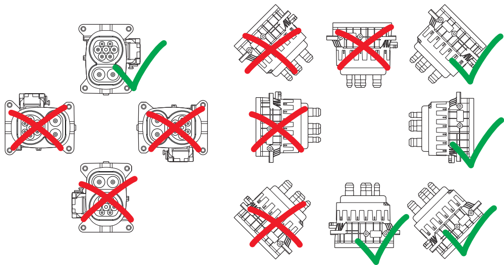
Connection diagram
