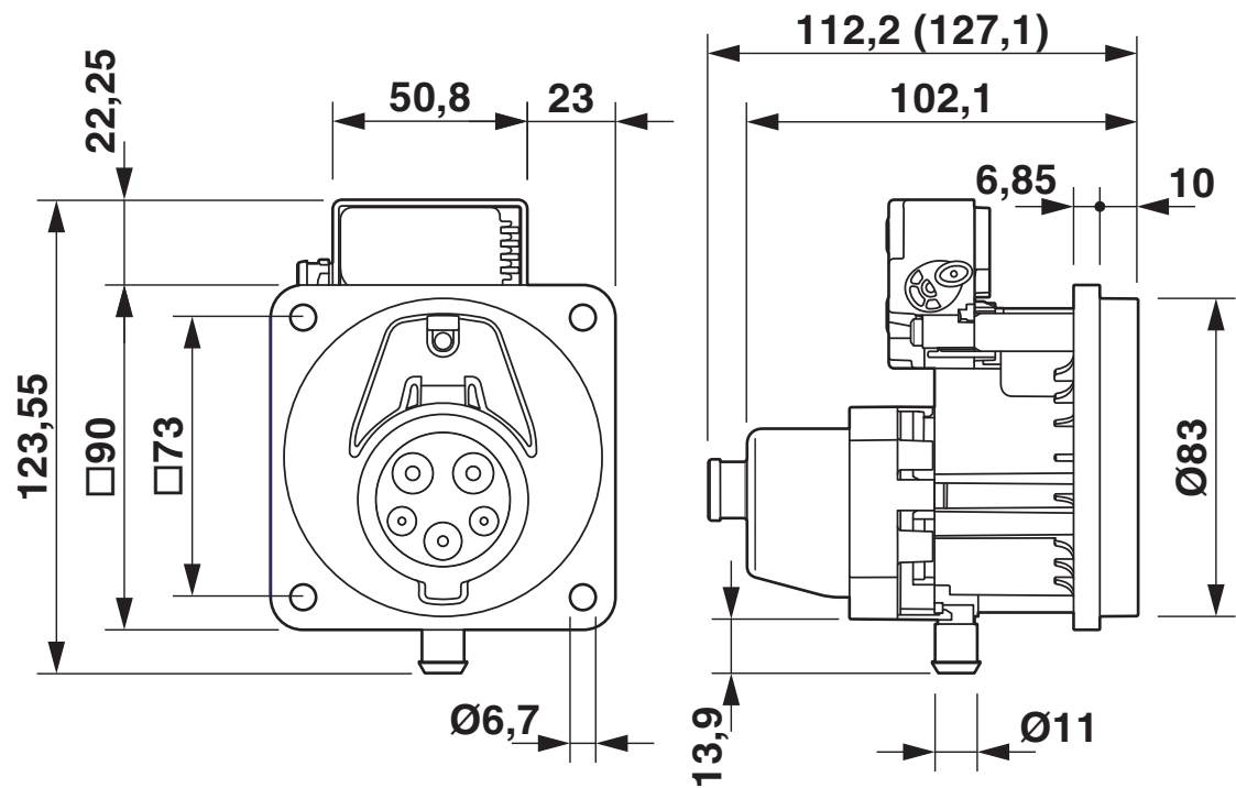
Dimensional drawing
