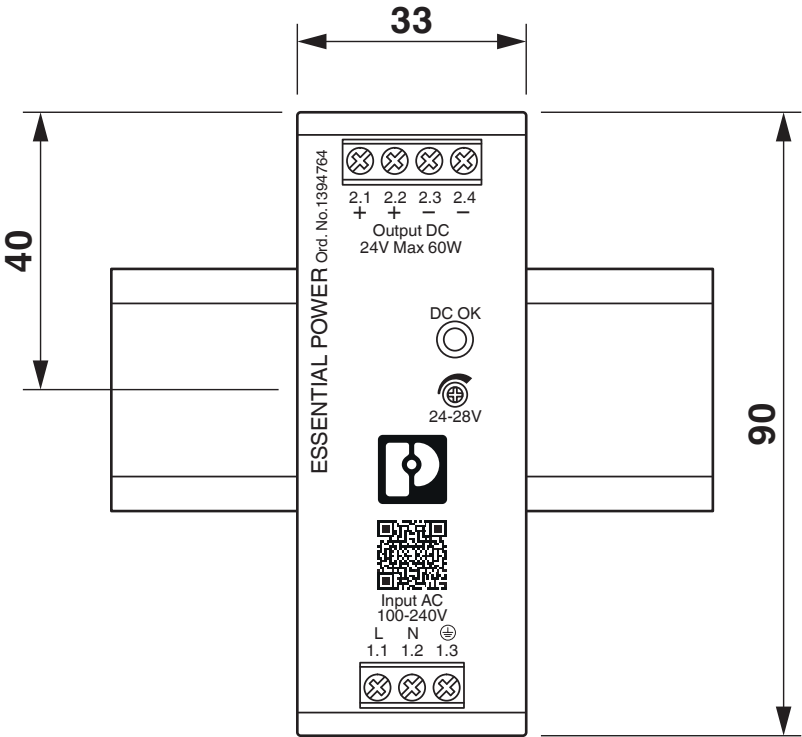
Dimensional drawing
