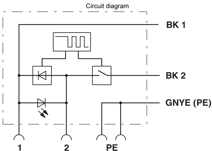
Valve connector connector pin assignment, type C
