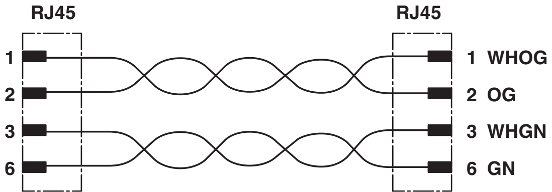
Circuit diagram
